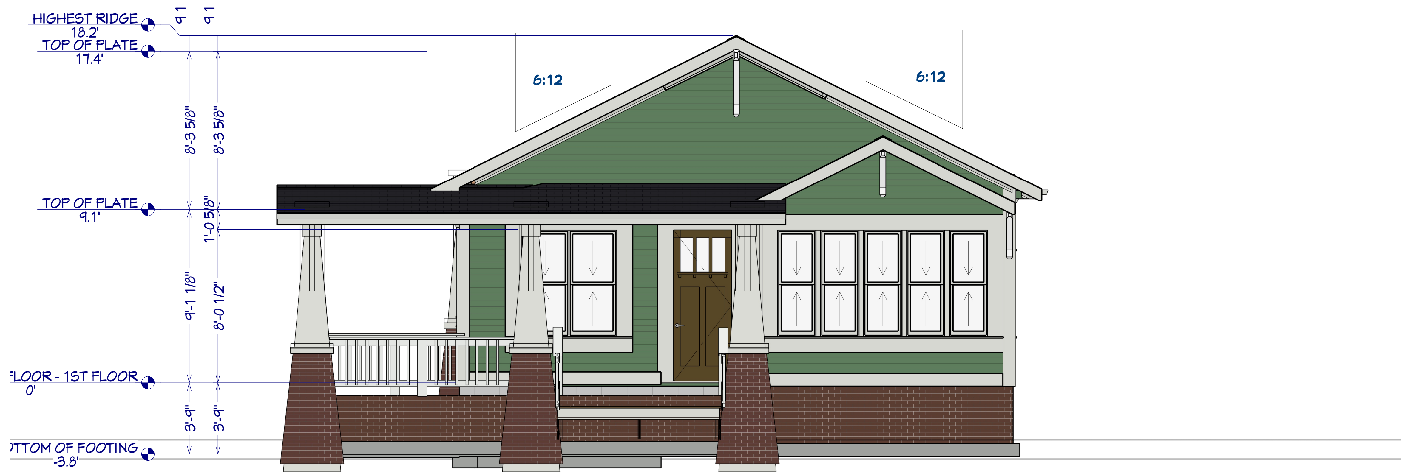
Front Elevation
