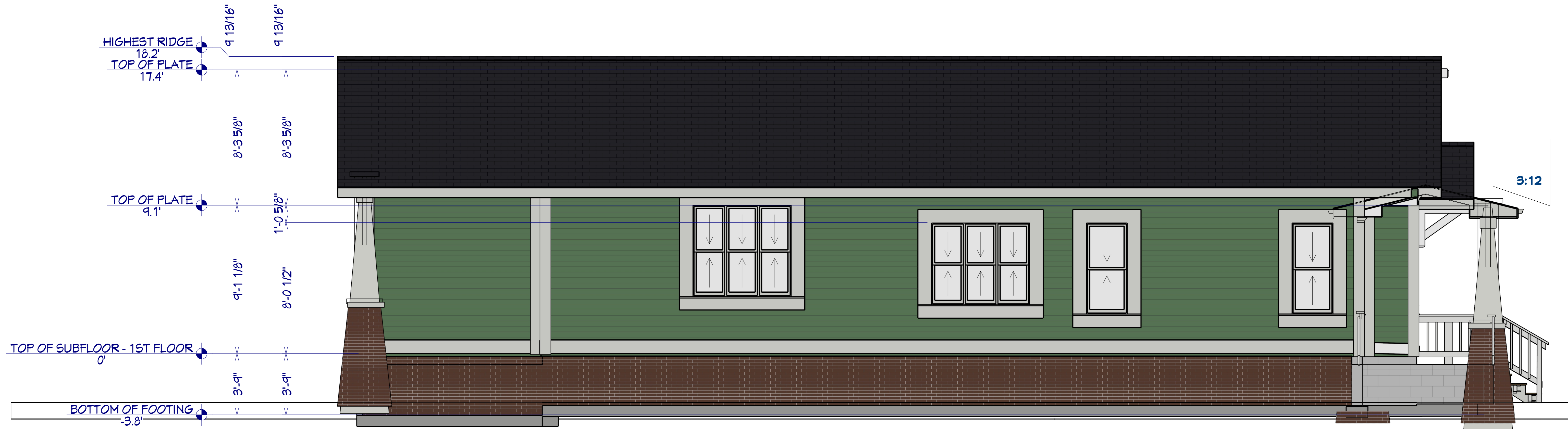
Left Elevation
