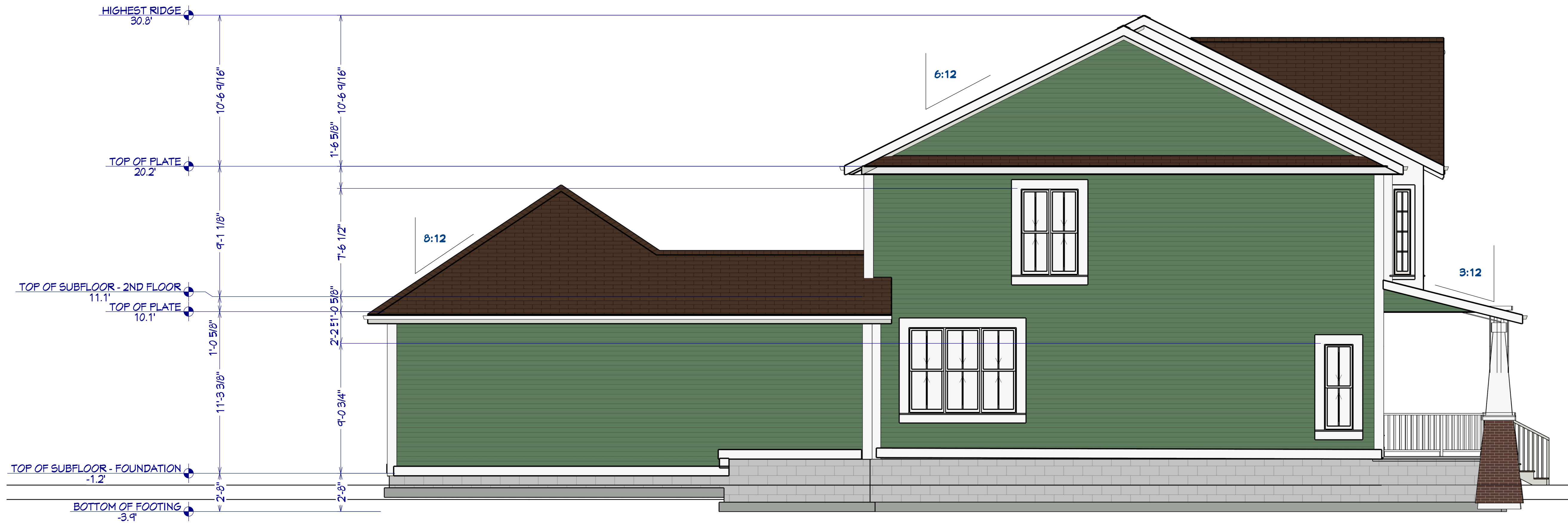
Left Elevation
