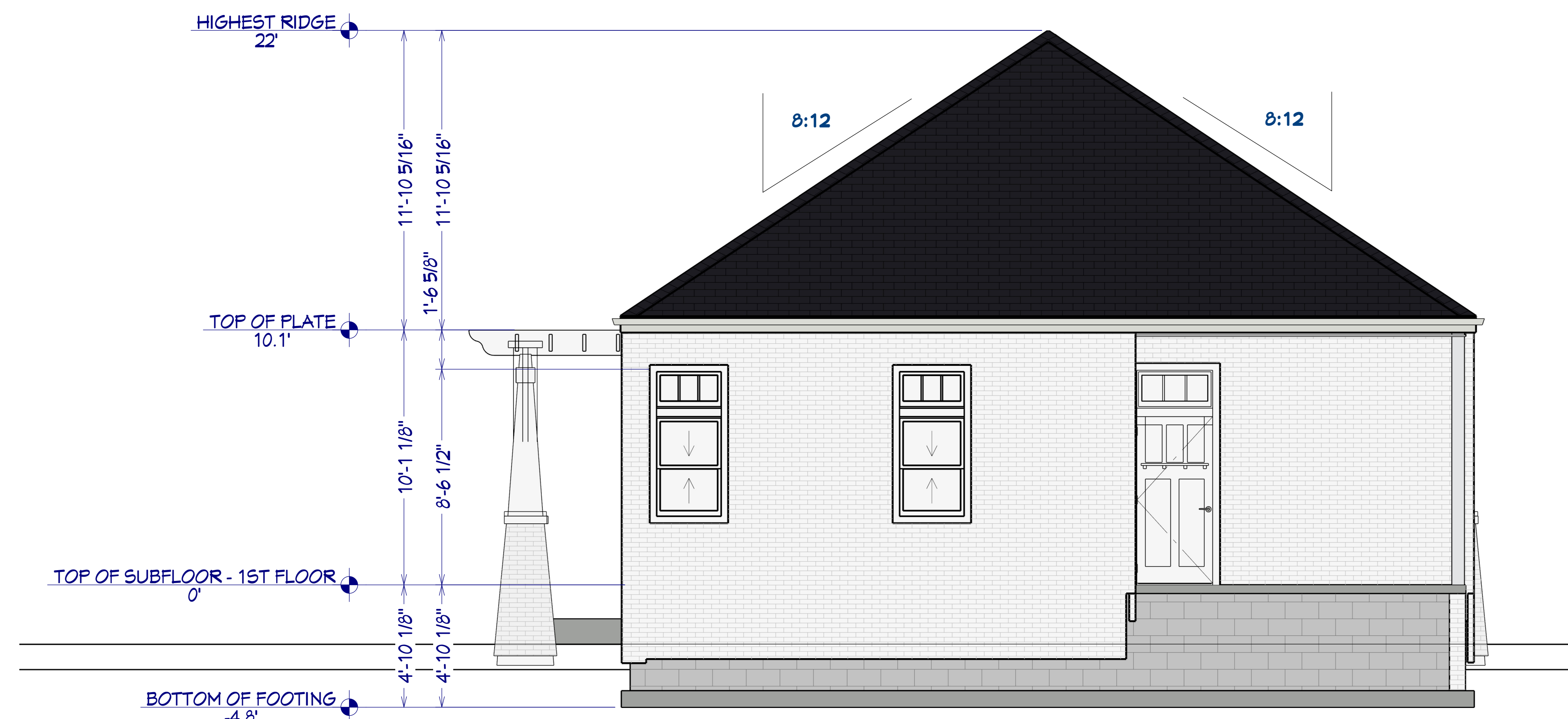
Rear Elevation
